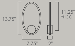
LOOP SM251422
