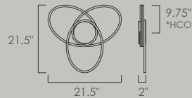
LOOP SM251423
